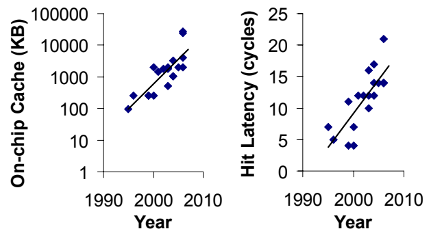
Figure 1. Historic trends of on-chip caches on (a) size, and (b) latency.
